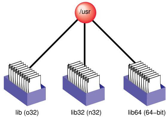
Figure 3-2 Library Locations for the Different ABIs
