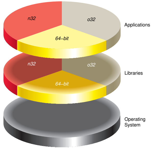
Figure 3-1 Application Support Under Different ABIs
